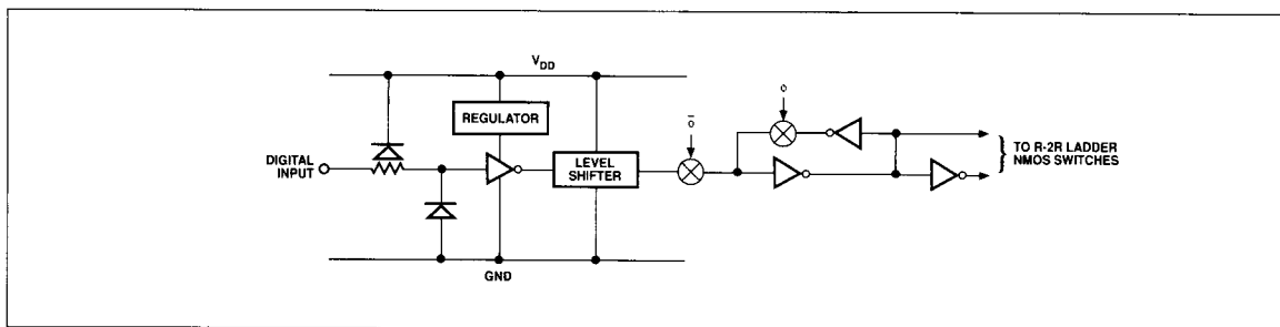
FIGURE 4: Simplified Digital Input Structure
