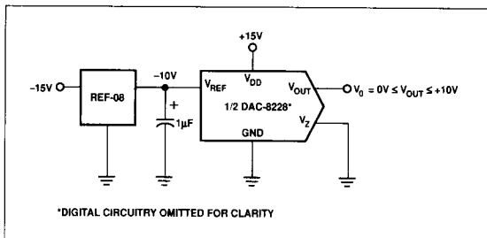
FIGURE 7: Single Supply Configuration ( 0V \leq V_{OUT} \leq +10V )
