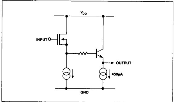
FIGURE 2: Amplifier Output Stage
