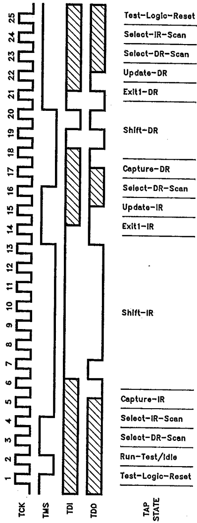
FIGURE 9. TIMING EXAMPLE
