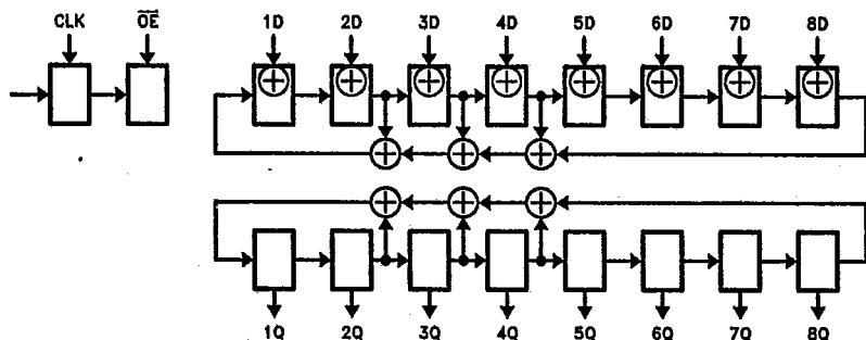
FIGURE 8. 8-BIT PSA AND PRPG CONFIGURATION
