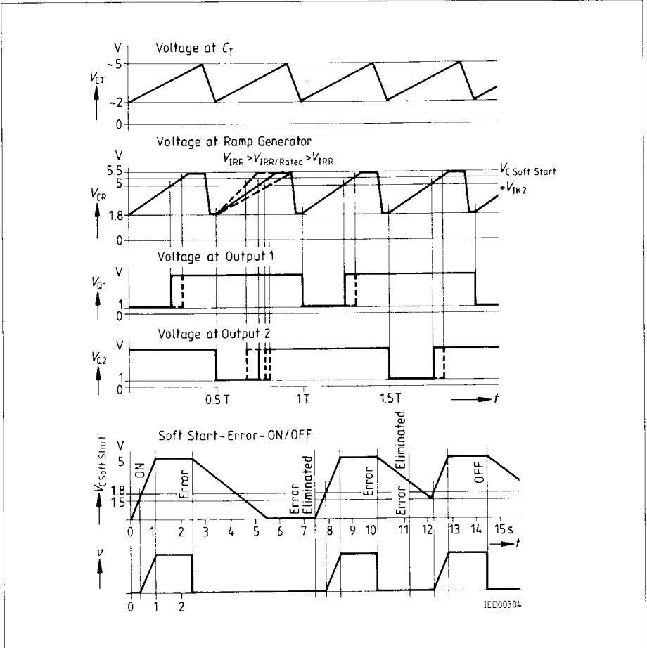
Pulse Diagram
