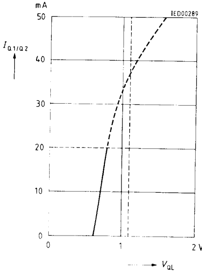
Output Current versus L-Output Voltage
