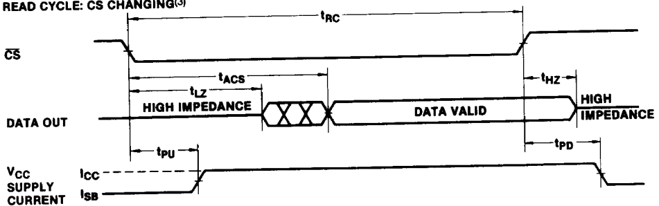
READ CYCLE: \overline{CS} CHANGING(3)
