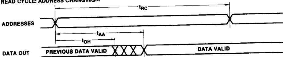
READ CYCLE: ADDRESS CHANGING(2)
