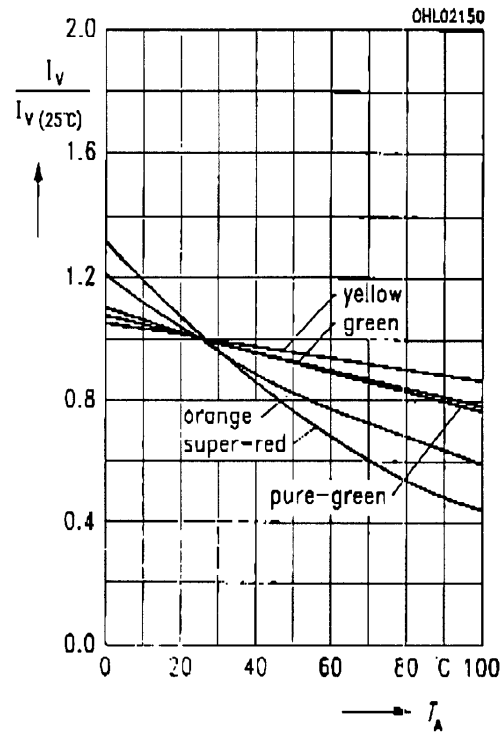
Relative Lichtstärke I_V / I_{V(25^\circ\text{C})} = f(T_A) Relative luminous intensity I_F = 10 \text{ mA}
