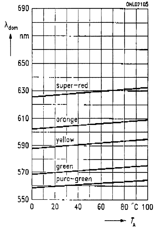
Dominantwellenlänge \lambda_{\text{dom}} = f(T_A) Dominant wavelength I_F = 10 \text{ mA}
