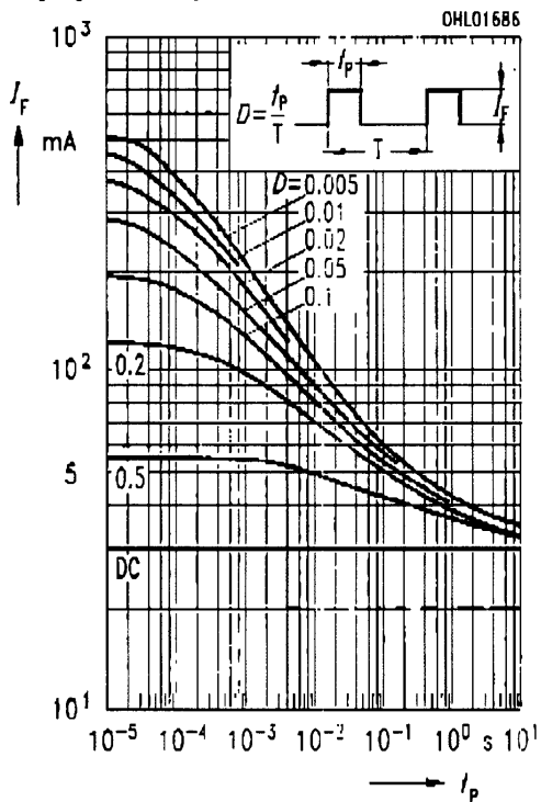
Zulässige Impulsbelastbarkeit I_F = f(t_p) Permissible pulse handling capability Duty cycle D = \text{parameter} , T_A = 25^\circ\text{C}
