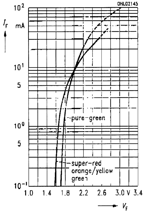
Durchlaßstrom I_F = f(V_F) Forward current T_A = 25^\circ\text{C}
