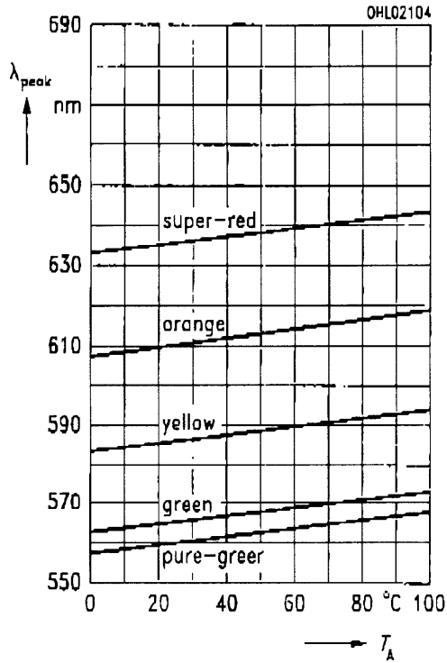
Wellenlänge der Strahlung \lambda_{\text{peak}} = f(T_A) Wavelength at peak emission I_F = 10 \text{ mA}
