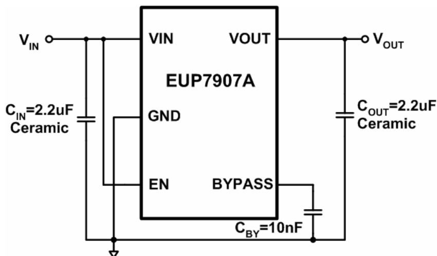
Figure. 1 Fixed Output
