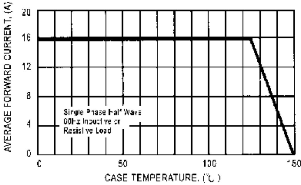
FIG. 2 - TYPICAL FORWARD CURRENT DERATING CURVE
