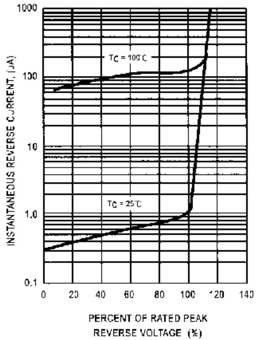
FIG. 3 - TYPICAL REVERSE CHARACTERISTICS
