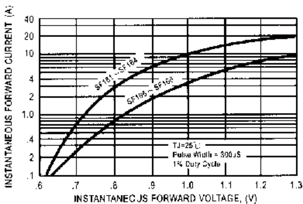
FIG. 5 - TYPICAL INSTANTANEOUS FORWARD CHARACTERISTICS
