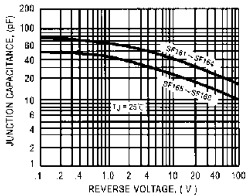
FIG. 6 - TYPICAL JUNCTION CAPACITANCE
