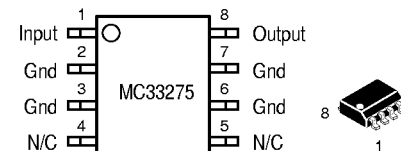
D SUFFIX PLASTIC PACKAGE CASE 751-06 (SOP-8)
