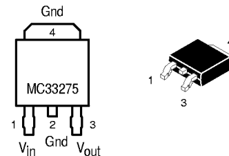
DT SUFFIX PLASTIC PACKAGE CASE 369A (DPAK)
