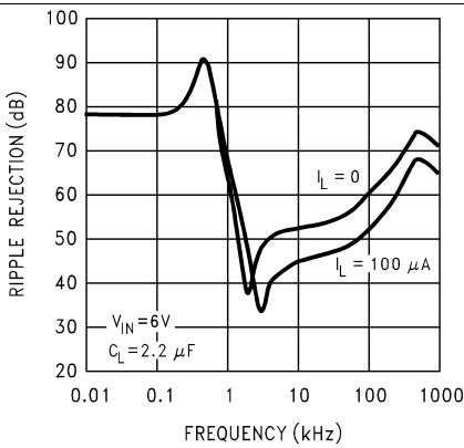
Figure 7. Ripple Rejection
