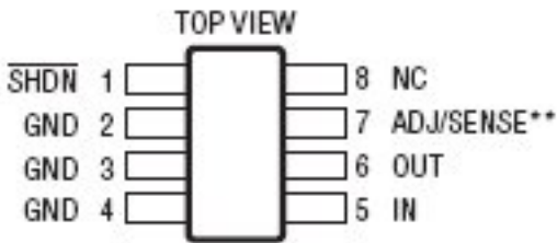
TS8 PACKAGE 8-LEAD PLASTIC TSOT-23
