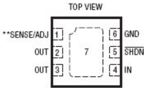
DC PACKAGE 6-LEAD (2mm × 2mm) PLASTIC DFN
