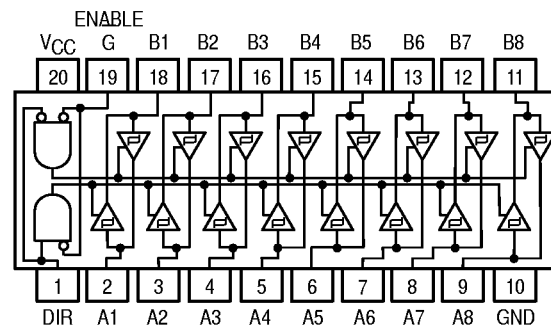
SN54/74LS641 SN54/74LS645
