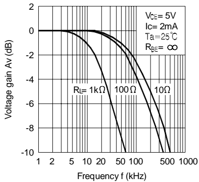
Fig.11 Frequency Response
