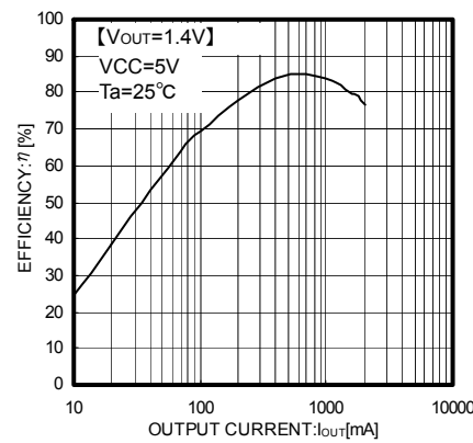
Fig.50 Efficiency
