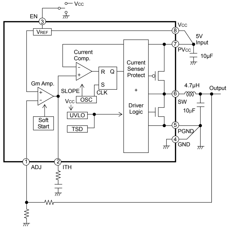
Fig.77 BD9106FVM, BD9107FVM Block Diagram
