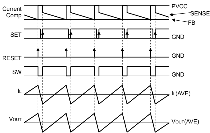
Fig.87 Diagram of current mode PWM control
