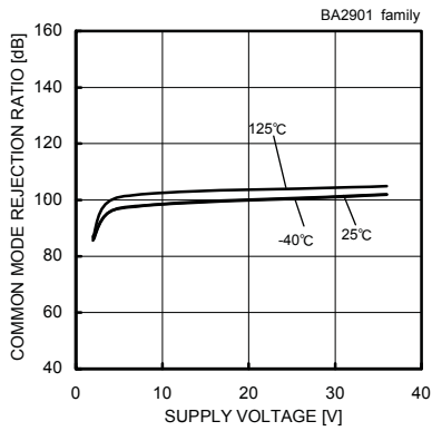
Fig. 16 Common Mode Rejection Ratio – Supply Voltage
