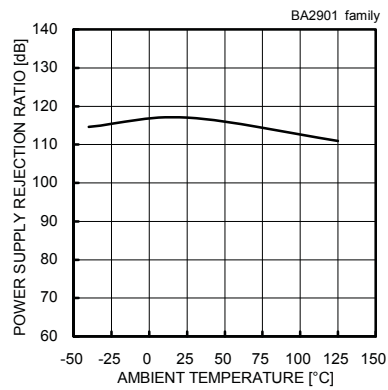
Fig. 19 Power Supply Rejection Ratio – Ambient Temperature
