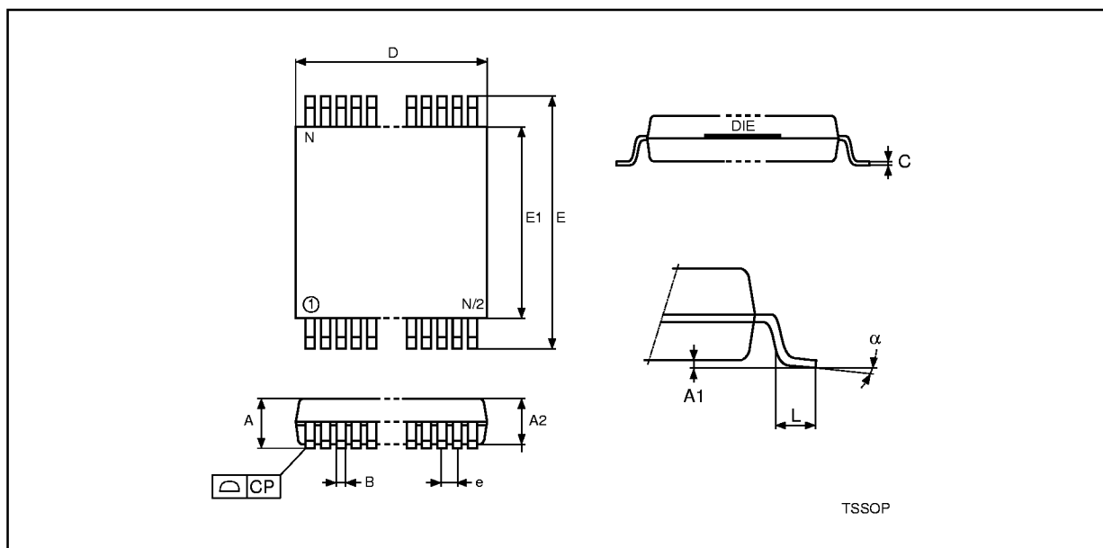
Figure 13. TSSOP14 (DL)
