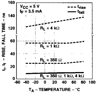
Figure 14. Typical Rise and Fall Time vs. Temperature.
