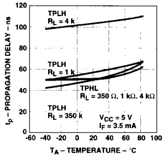
Figure 11. Typical Propagation Delay vs. Temperature.
