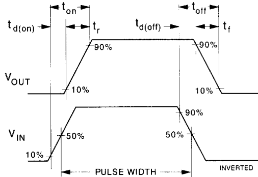
Figure 12. Switching Waveforms.
