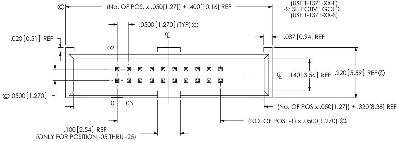
FIG 1 (ESHF-110-01-X-D-TH-LC SHOWN)
