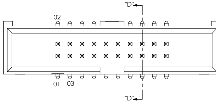
FIG 3 (ESHF-110-01-X-D-SM-LC SHOWN) (SAME AS FIG 1, DIFFERENT AS SHOWN)
