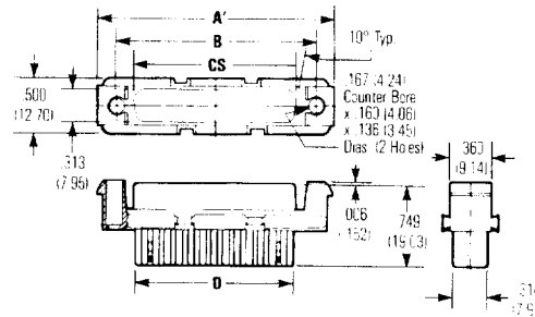
Socket with Latching Blocks
