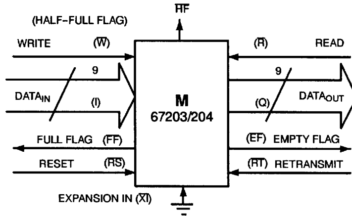
Figure 2. Block Diagram of Single 2K x 9 and 4K x 9 FIFO.
