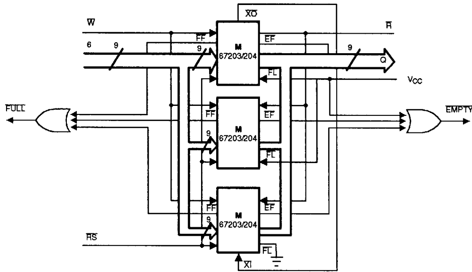
Figure 4. Block Diagram of 6144 x 9 / 12288 x 9 FIFO Memory (Depth expansion).
