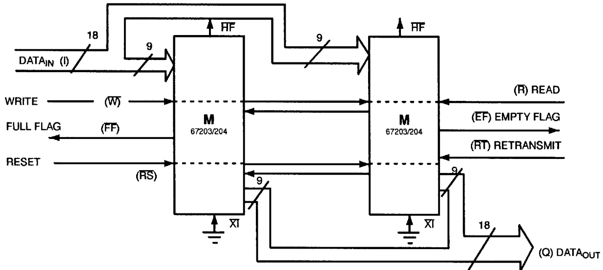
Figure 3. Block Diagram of 2048 / 4096 x 18 FIFO Memory Used in Width Expansion Mode.
