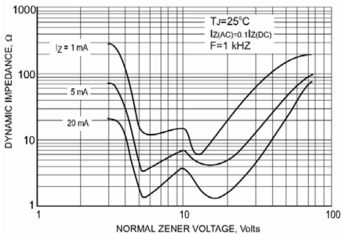
Fig.5 EFFECT OF ZENER VOLTAGE ON ZENER IMPEDANCE
