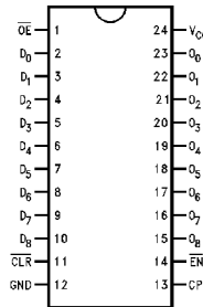
Pin Assignment for DIP and SOIC
