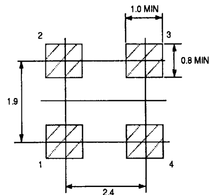
PACKAGE OUTLINE 39 RECOMMENDED P.C.B. LAYOUT
