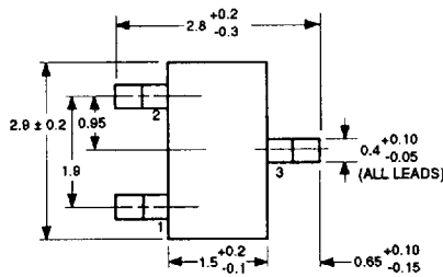
PACKAGE OUTLINE 33
