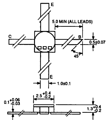
PACKAGE OUTLINE 07
