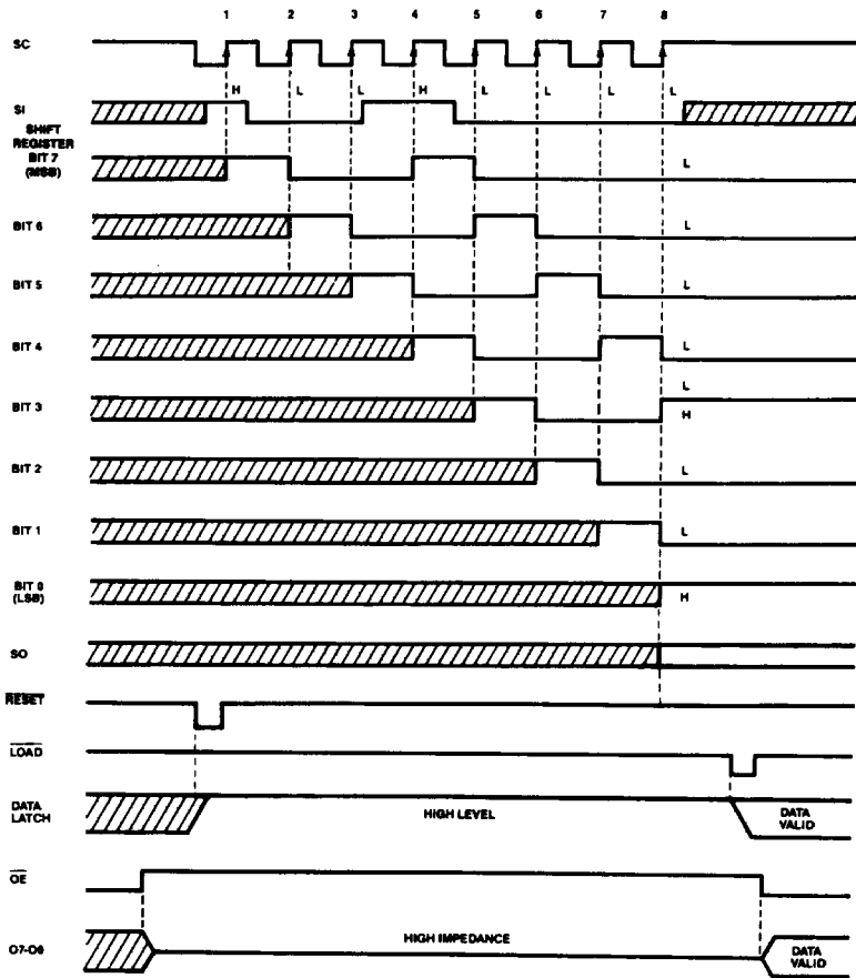
Figure 3. Input/Output Timing Based on the Rising Edge of SC (I/O timing for \overline{SC} is identical, except for pulse-width offset.)
