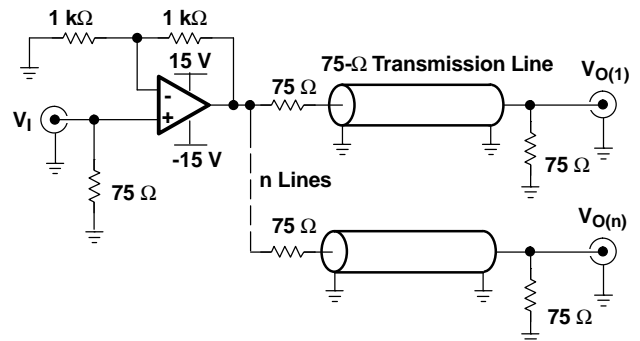
Figure 54. Video Distribution Amplifier Application
