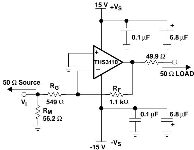
Figure 52. Wideband, Inverting Gain Configuration
