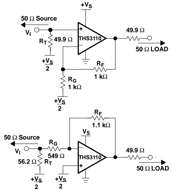
Figure 53. DC-Coupled, Single-Supply Operation
