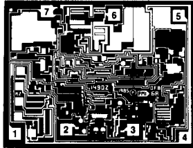
DIE SIZE 0.086 × 0.067 inch, 5762 sq. mils (2.18 × 1.70mm, 3.71 sq. mm)
