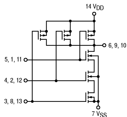
MC14023UB CIRCUIT SCHEMATIC (1/3 of Device Shown)
