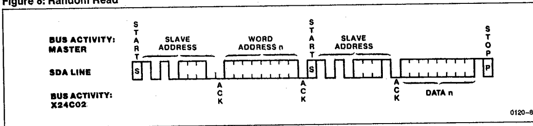
Figure 8: Random Read
