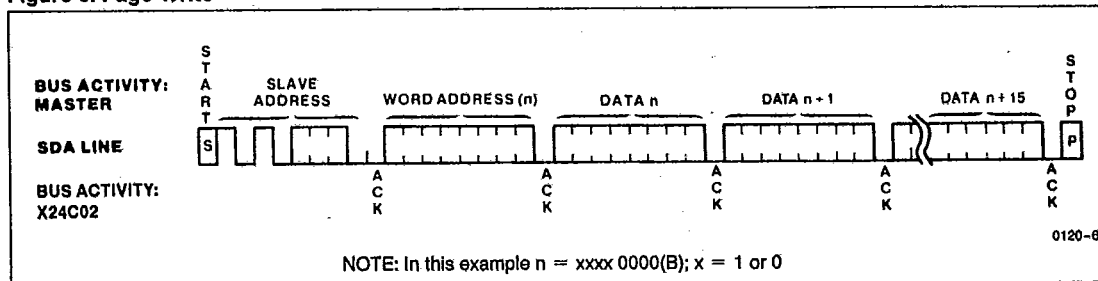
Figure 6: Page Write
