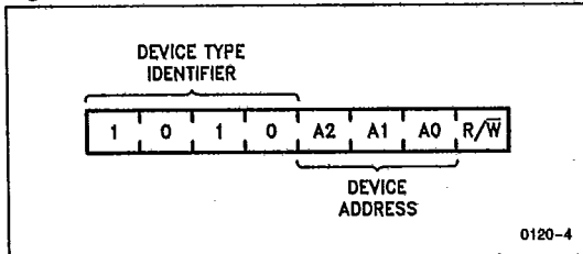
Figure 4: Slave Address
