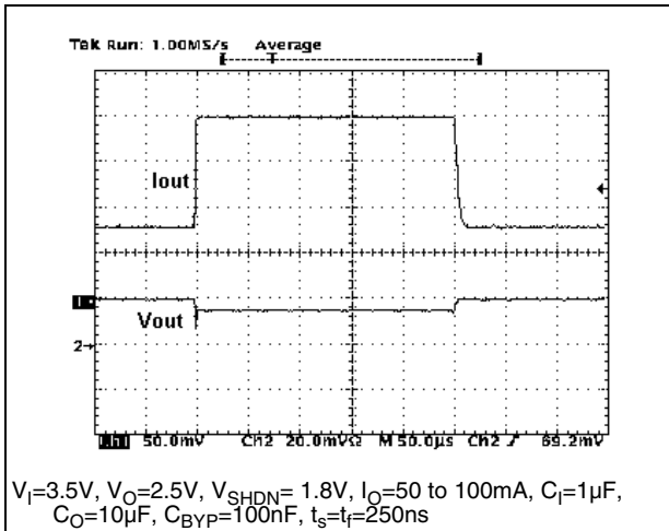
Figure 29. Load transient
