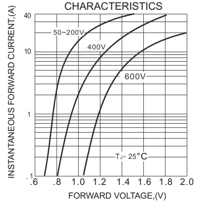
FIG.3-TYPICAL FORWARD CHARACTERISTICS
