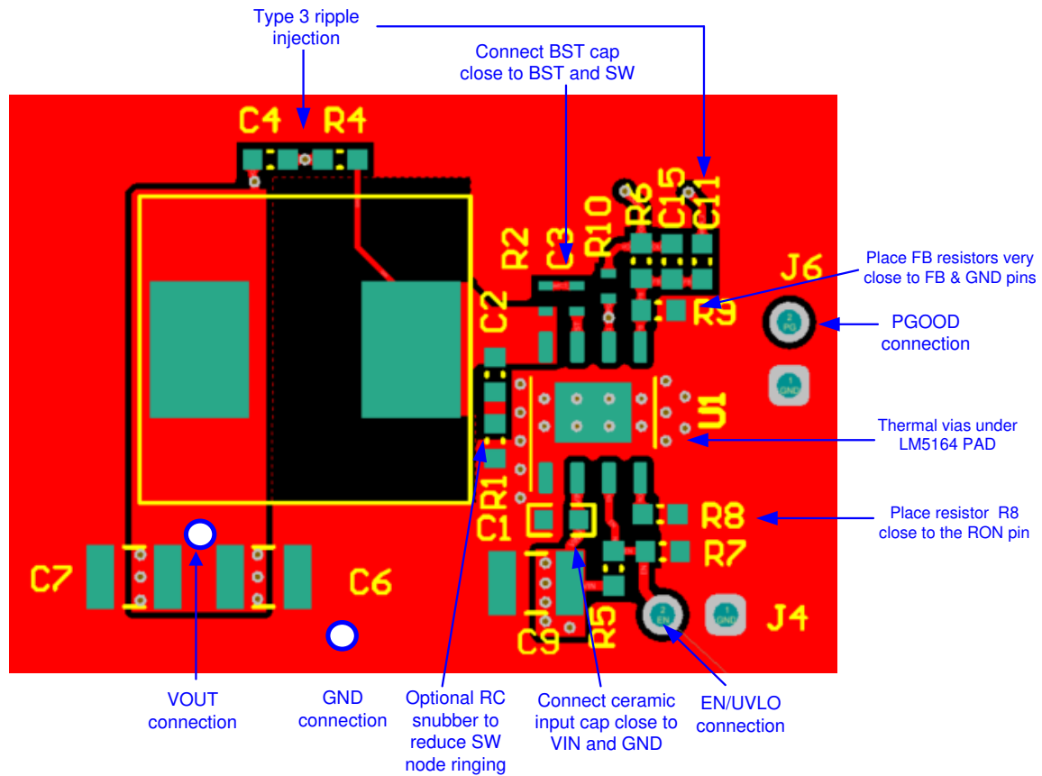
Figure 10-2. LM5164 Single-Sided PCB Layout Example
