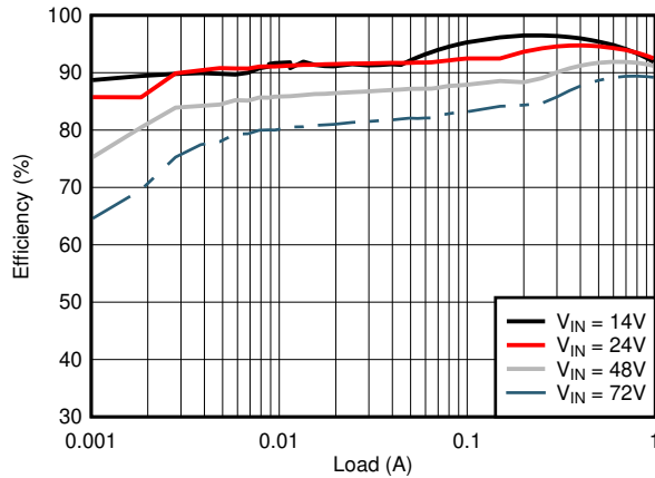
Figure 8-2. Conversion Efficiency (Log Scale)
