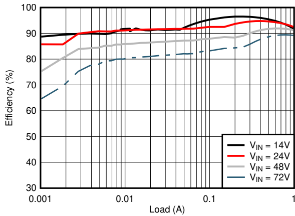
Figure 6-1. Conversion Efficiency (Log Scale)
