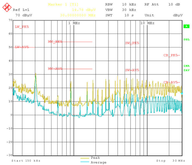
Figure 8-14. No-Load Switching
