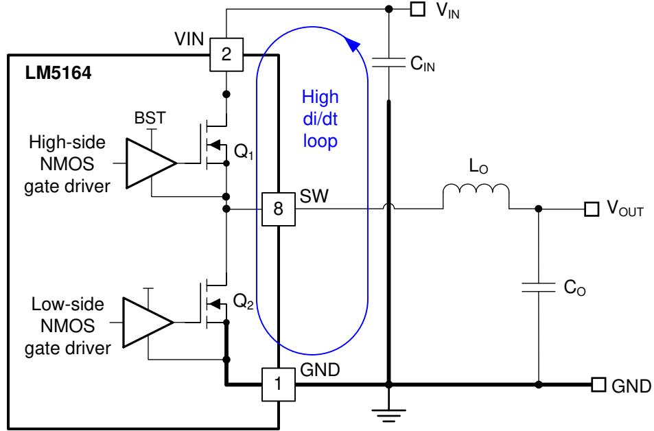
Figure 10-1. DC/DC Buck Converter With Power Stage Circuit Switching Loop
