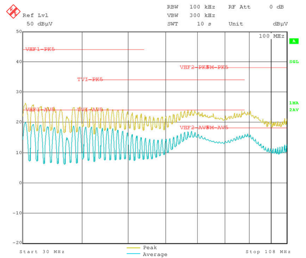
Figure 8-15. Full-Load Switching
