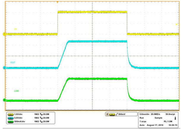
Figure 8-9. Full-Load Start-up and Shutdown with EN/UVLO
