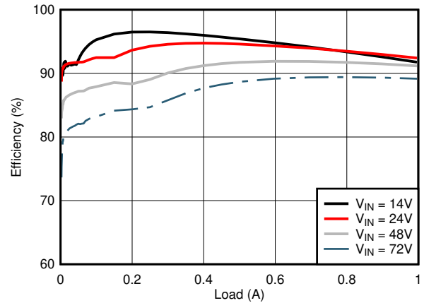
Figure 8-3. Conversion Efficiency (Linear Scale)
