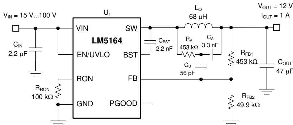
Figure 8-1. Typical Application V_{IN(nom)} = 48\text{ V} , V_{OUT} = 12\text{ V} , I_{OUT(max)} = 1\text{ A} , F_{SW(nom)} = 300\text{ kHz}
