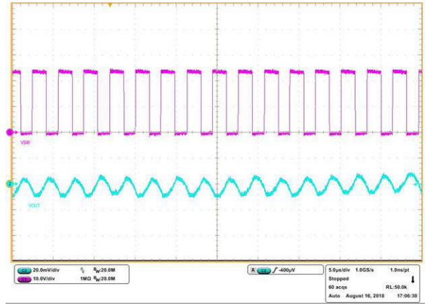
Figure 8-15. Full-Load Switching
