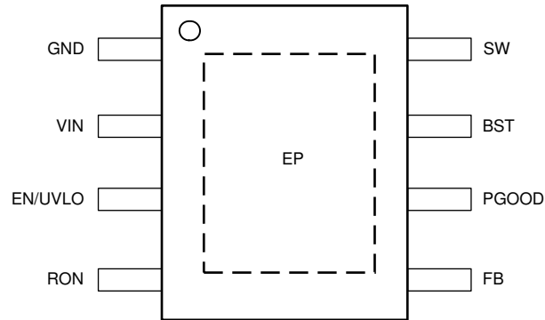
Figure 5-1. DDA Package 8-Pin SO PowerPAD Top View
