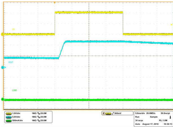
Figure 8-8. No-Load Start-up and Shutdown with EN/UVLO
