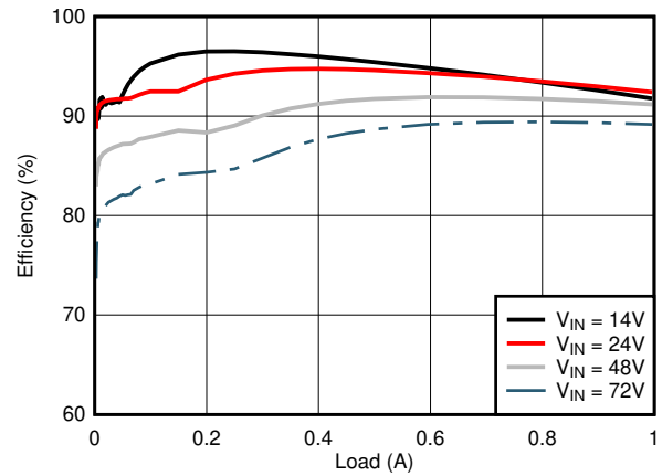
Figure 6-2. Conversion Efficiency (Linear Scale)
