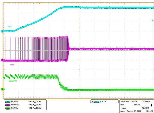
Figure 8-10. Pre-bias Start-up with EN/UVLO
