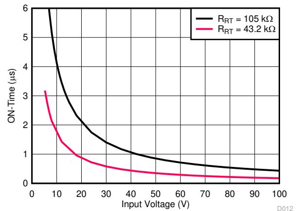
Figure 6-10. COT On-Time versus V_{IN}
