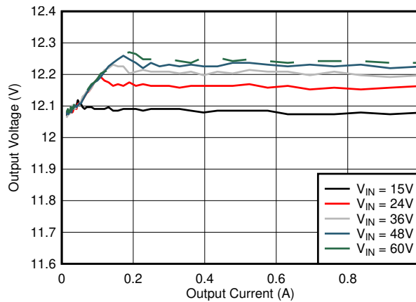
Figure 8-4. Load and Line Regulation Performance
