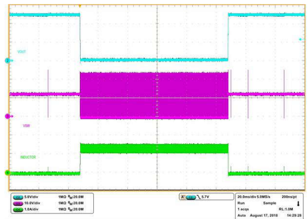
Figure 8-11. Short Circuit Applied
