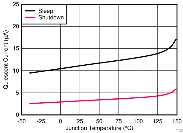
Figure 6-3. V_{IN} Shutdown and Sleep Supply Current versus Temperature
