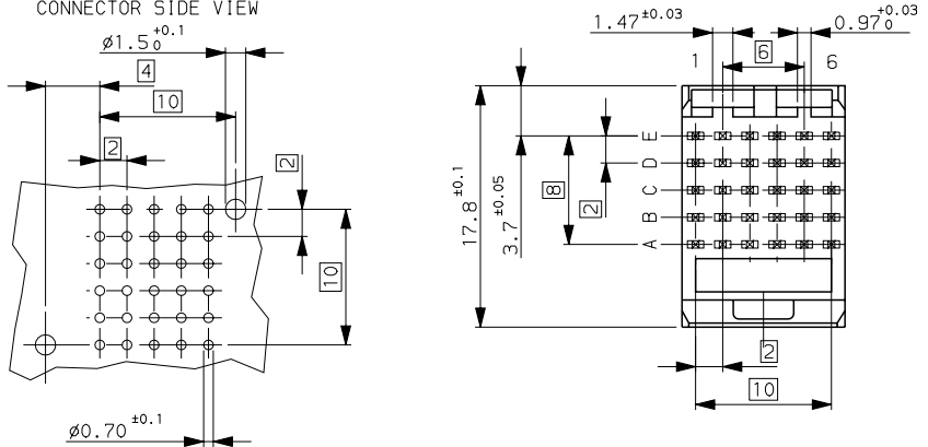
LAYOUT FOR P.C.B (PER 12mm LENGTH)
