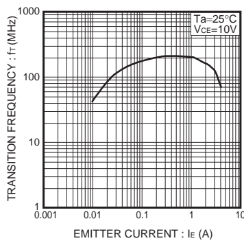
Fig.8 Transition frequency
