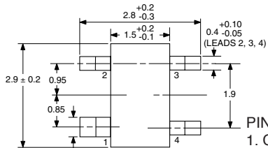
PACKAGE OUTLINE 39
