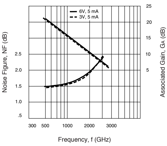
NE68018 NOISE FIGURE & ASSOCIATED GAIN vs. FREQUENCY
