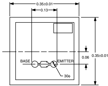
NE68000 (CHIP) (Chip Thickness: 160 μm)
