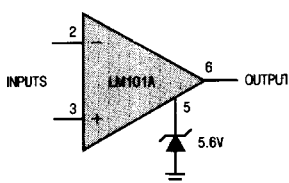
Voltage Comparator with Clamp
