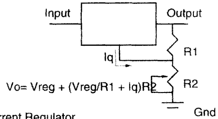
Current Regulator
