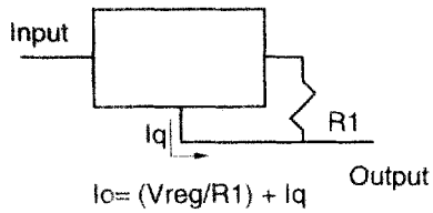
Current Regulator
