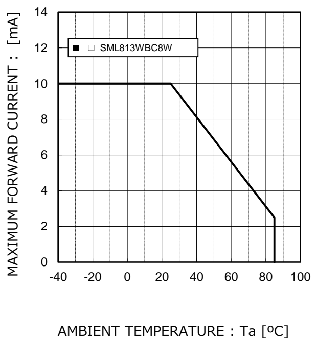
Fig.4 Derating
