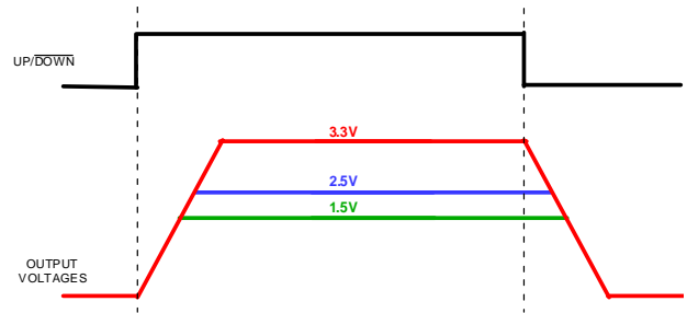
Figure 1. ADM1200-1 Power-Up and Power-Down Waveforms
