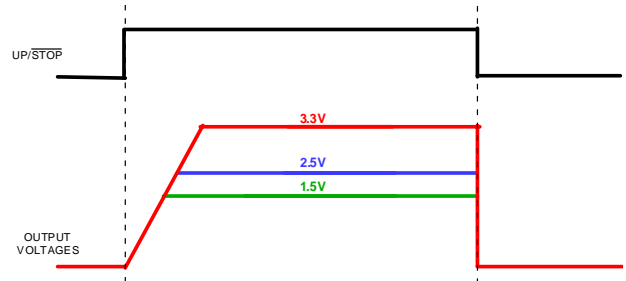
Figure 2. ADM1200-2 Power-Up and Power-Down Waveforms
