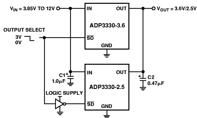
Figure 24. Crossover Switch
