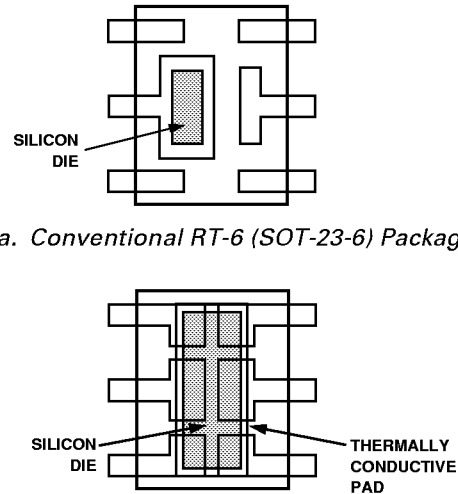
Figure 22. a. Conventional RT-6 (SOT-23-6) Package b. Chip-On-Lead Package
