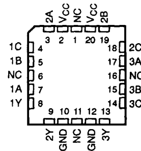
54AC11010 . . . FK PACKAGE (TOP VIEW)
