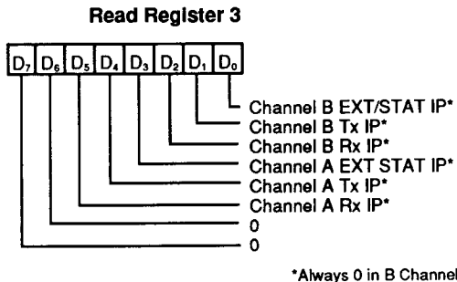
Figure 7. Read Register Bit Functions
