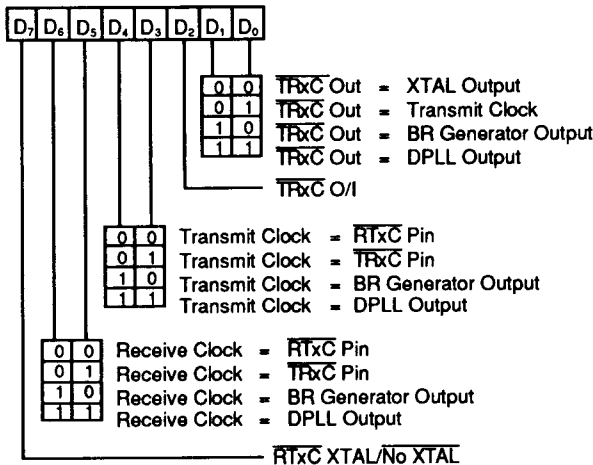
Figure 8. Write Register Bit Functions (continued)
