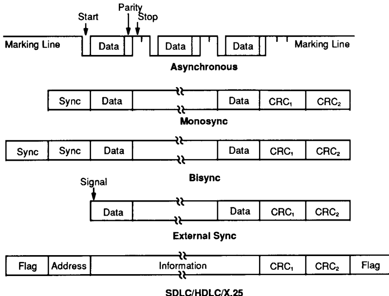
Figure 2. SCC Protocols
