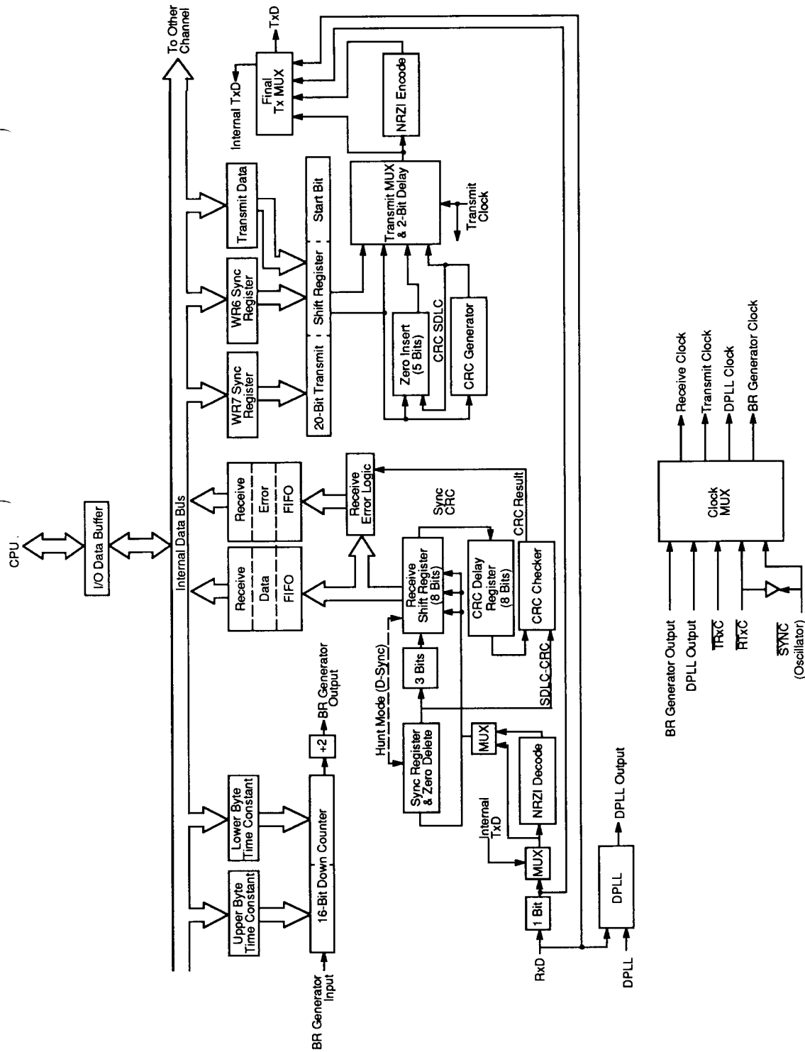
Figure 1. Data Path
