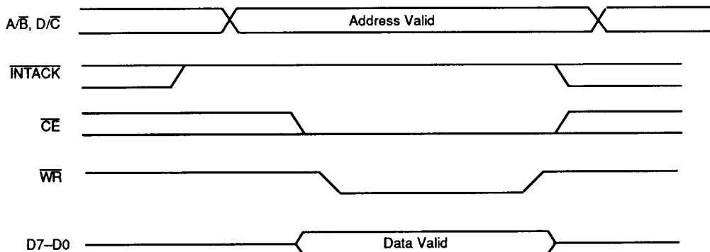
Figure 12. Read Cycle Timing
