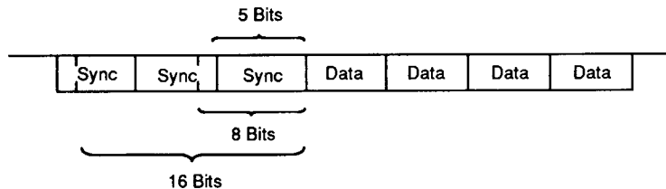
Figure 3. Detecting 5- or 7-Bit Synchronous Characters
