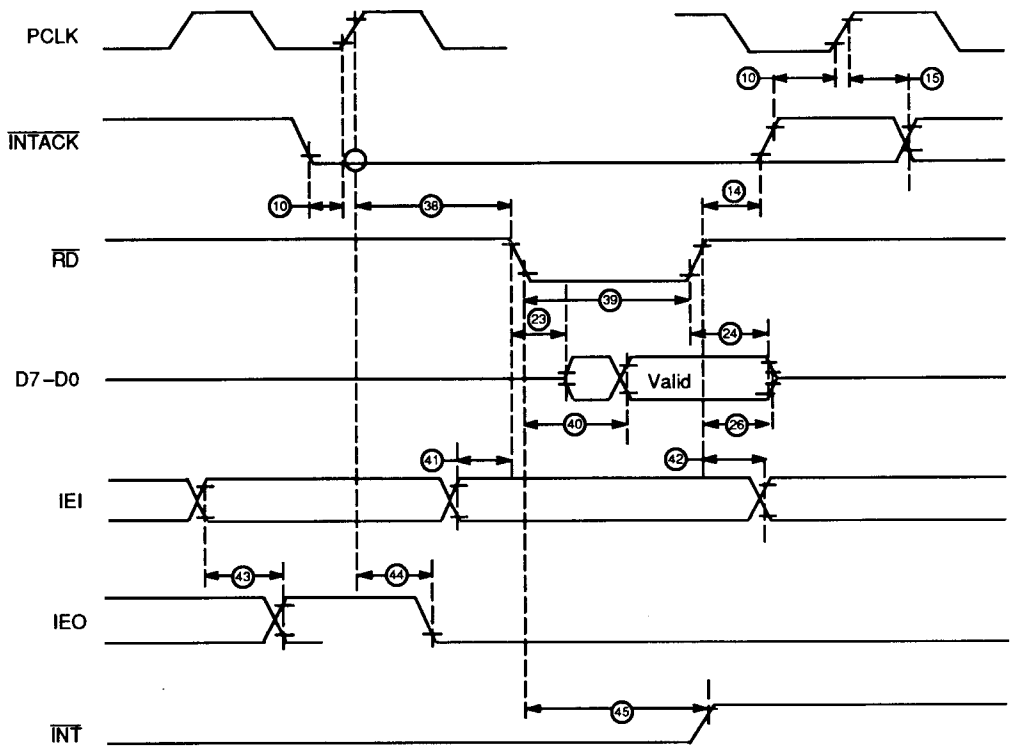
Figure 22. Interrupt Acknowledge Timing (Am8530)
