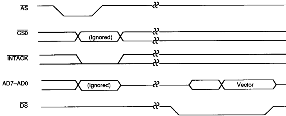
Figure 11. Interrupt Acknowledge Cycle Timing
