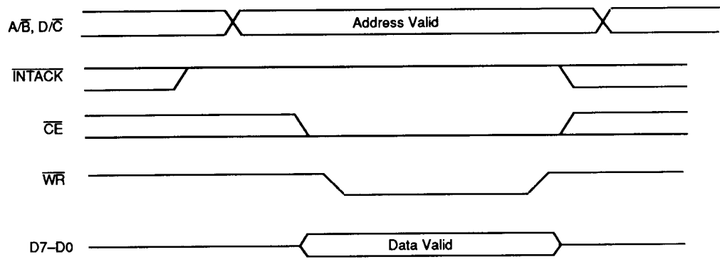
Figure 13. Write Cycle Timing
