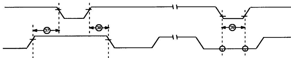
Figure 20. Reset Timing (Am8030)
