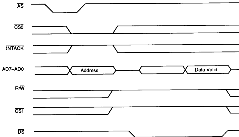
Figure 9. Read Cycle Timing
