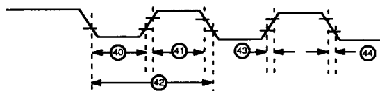
Figure 21. Cycle Timing (Am8030)
