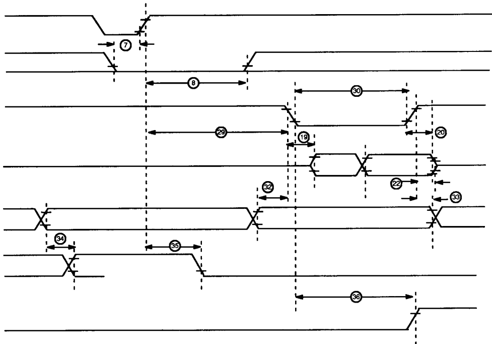
Figure 19. Interrupt Acknowledge Timing (Am8030)
