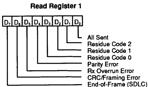
Figure 7. Read Register Bit Functions
