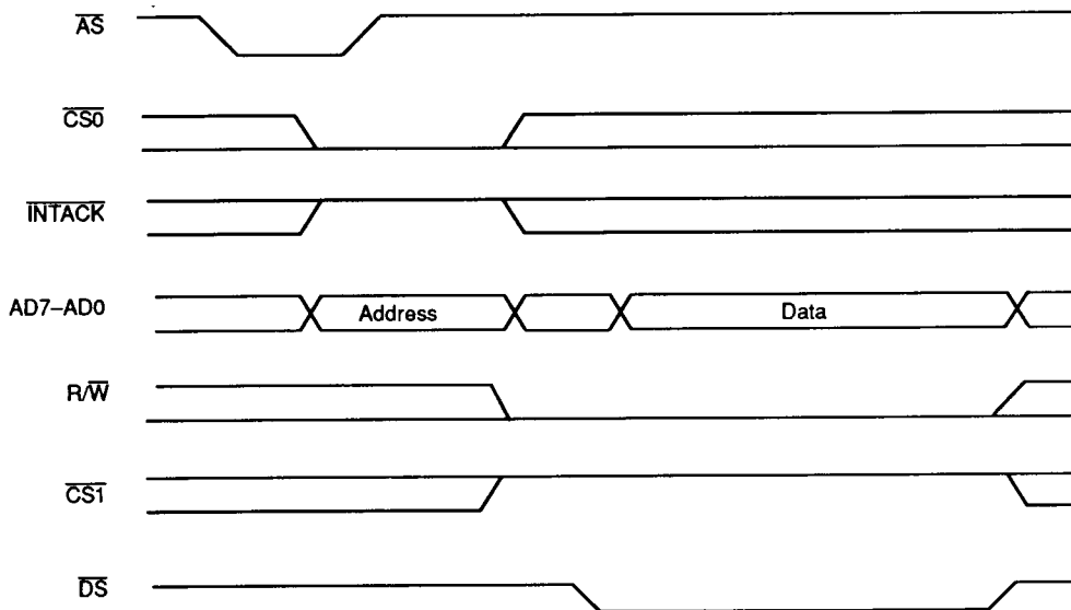
Figure 10. Write Cycle Timing
