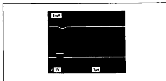
FIGURE 2C: Pulse Response with Output Decoupling
