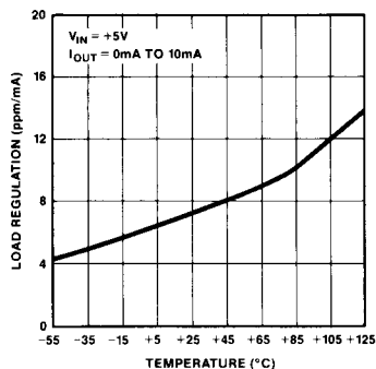
LOAD REGULATION vs TEMPERATURE
