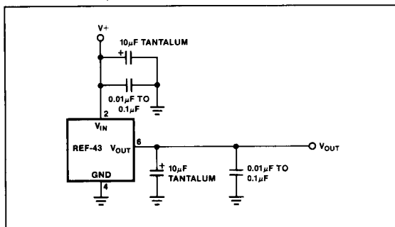
FIGURE 2A: Recommended Decoupling for High-Frequency Pulse Response
