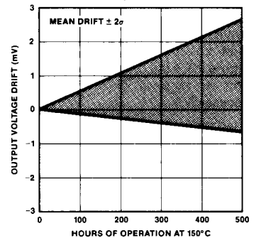
BURN-IN DRIFT AT TA = 150°C
