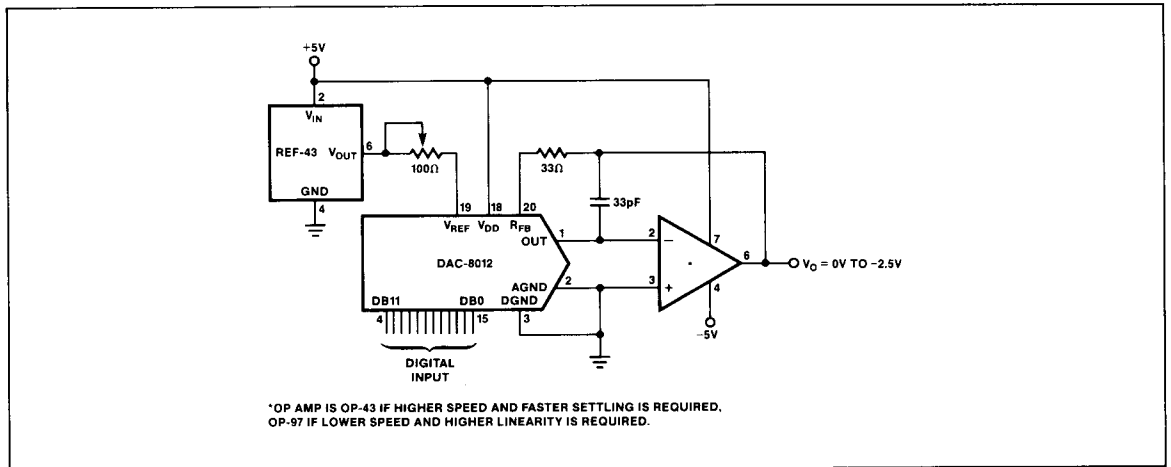
FIGURE 6: CMOS DAC Reference
