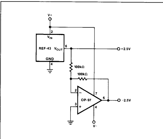
FIGURE 3: \pm 2.5\text{V} Reference
