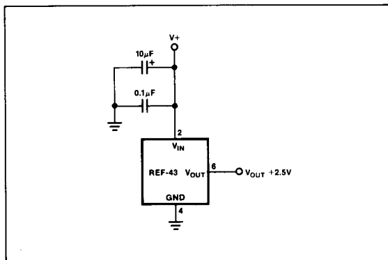
FIGURE 1: Basic Connections
