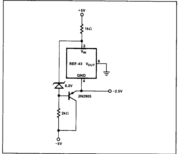
FIGURE 4: -2.5V Reference
