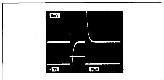
FIGURE 2B: Pulse Response with No Output Decoupling
