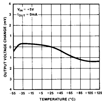
OUTPUT VOLTAGE CHANGE vs TEMPERATURE
