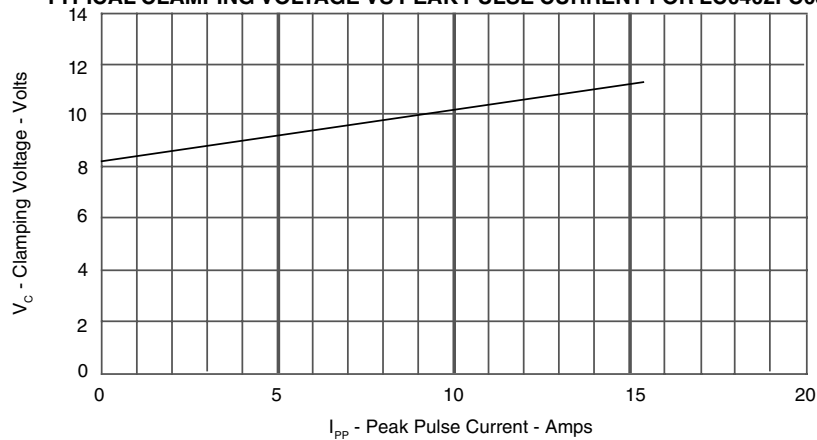
FIGURE 5 TYPICAL CLAMPING VOLTAGE VS PEAK PULSE CURRENT FOR LC0402FC05C
