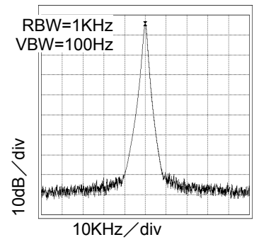
Fig.48 27MHz Spectrum VDD=3.3V, at CL=40pF
