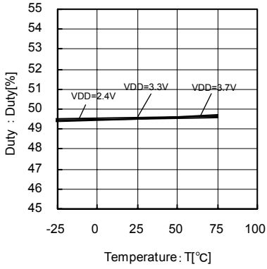
Fig.99 33.9MHz Temperature - Duty
