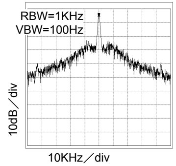
Fig.81 33.9MHz Spectrum VDD=3.3V, at CL=15pF
