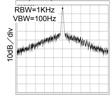
Fig.90 24.6MHz Spectrum VDD=3.3V, at CL=15pF
