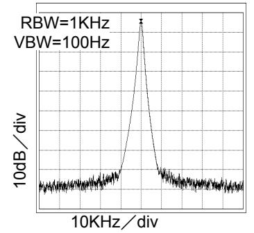
Fig.51 27MHz Spectrum VDD=3.3V, at CL=25pF
