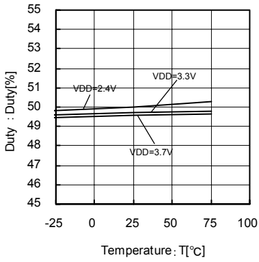
Fig.102 36.9MHz Temperature - Duty
