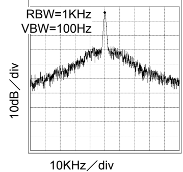
Fig.87 22.6MHz Spectrum VDD=3.3V, at CL=15pF
