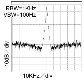
Fig.60 22.6MHz Spectrum VDD=3.3V, at CL=15pF
