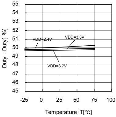
Fig.105 22.6MHz Temperature - Duty
