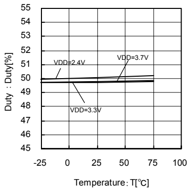
Fig.108 24.6MHz Temperature - Duty
