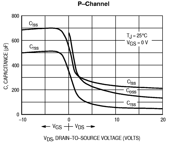
Figure 7. Capacitance Variation
