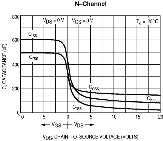
Figure 7. Capacitance Variation
