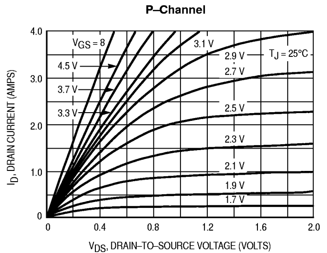
Figure 1. On-Region Characteristics
