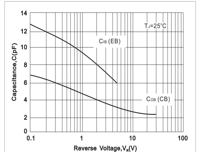
Fig.2- TYPICAL CAPACITANCES vs. REVERSE VOLTAGE
