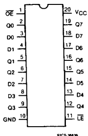
CD54/74AC373, CD54/74ACT373
