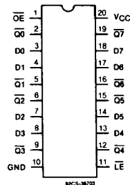
CD54/74AC533, CD54/74ACT533
