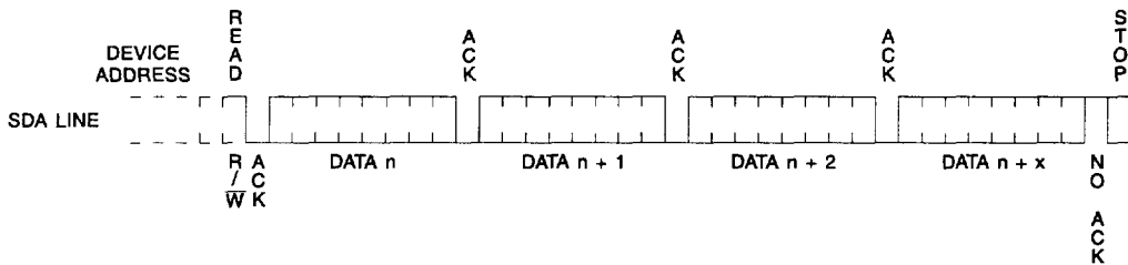
Figure 6. Sequential Read
