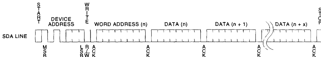
Figure 3. Page Write
