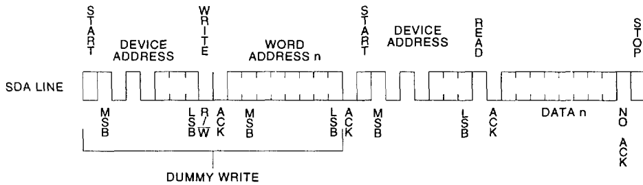
Figure 5. Random Read
