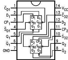
Pin Assignment for DIP, SOIC and TSSOP
