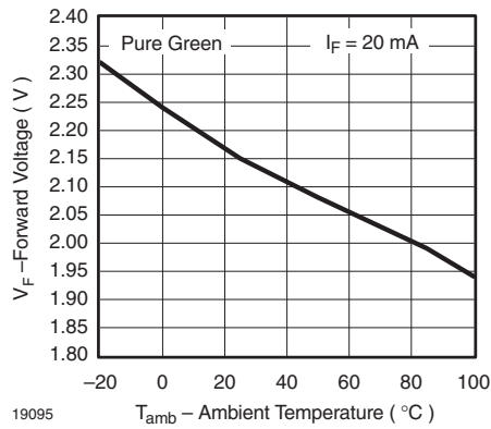
Figure 17. Forward Voltage vs. Ambient Temperature
